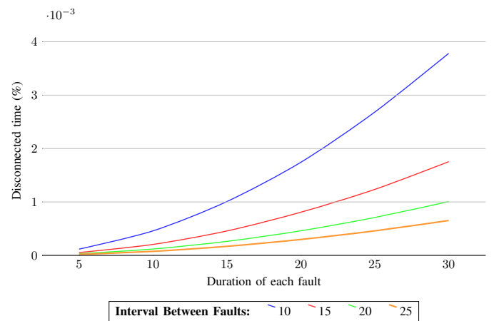
Fig. 7. Reliability vs Failure Duration and Frequency – Germany50 average
