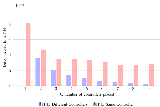
Fig. 5. Disconnection per controller number – disjoint paths versus separate controllers – Polska average
