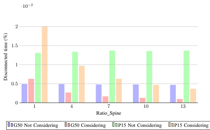
Fig. 3. Disconnection percentage when considering or not the differential availability in the network when placing controllers – averages for Germany50 (G50) and Polska (P15) networks
