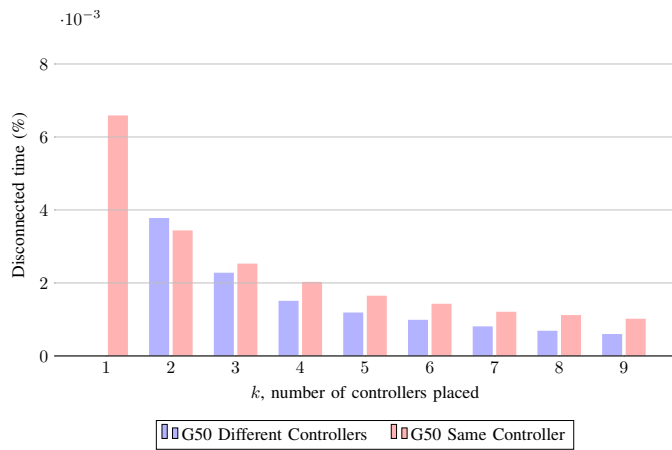
Fig. 4. Disconnection per controller number – disjoint paths versus separate controllers – Germany50 average
