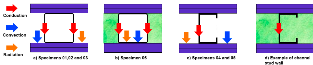
Figure 6.1 - Heat transfer mechanism in the hollow section and channel with and without insulation.
