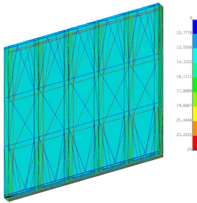
Figure 4.15 - Convective coefficients scheme applied to surfaces of hollow section specimens without wall cavity insulation.
