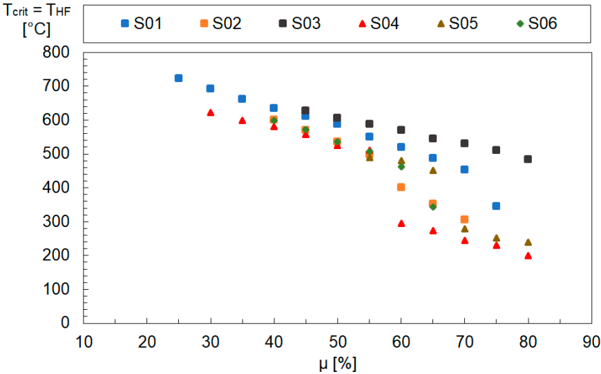
Figure 5.2 - Critical Temperature of the steel stud for all specimens
