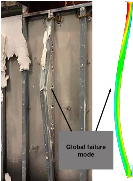
Figure 4.43 – Critical failure modes of stud 4 from fire test specimen [9] and stud 4 at failure time from FEM.
