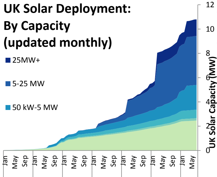
Figure 3 - UK Solar PV deployment by capacity (GOV.UK, 2016)
