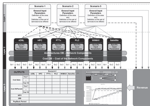
Fig 2. Tool architecture (layers)
