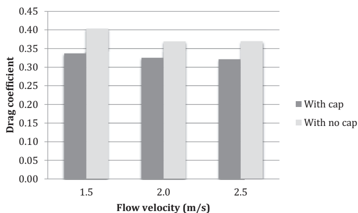
Figure 2: Values of drag coefficient for the female swimmer's model with cap and with no cap.
