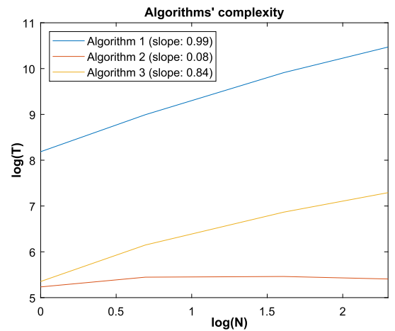
Fig. 9. Complexity from the three algorithms based on the big-o annotation. T represents the time consumed to iterate the input of size N.
