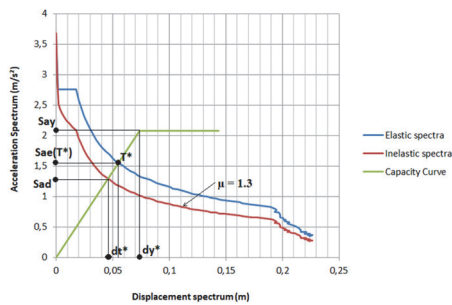
Figure 3: Capacity Curve VS Acceleration
