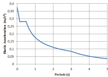
Figure 1: Elastic Response Spectrum
