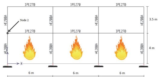
Figure 2: Fire scenario and portal frame
