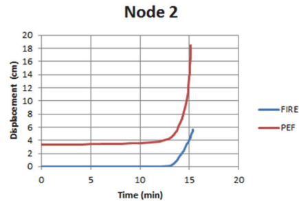
Figure 4: Local horizontal displacement
