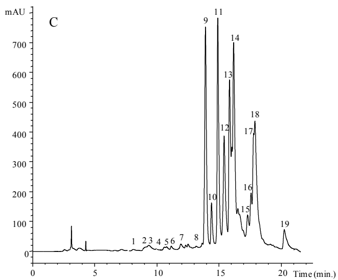
Figure 1. Individual chromatograms of the studied wild flowers: A- Castanea sativa ; B- Filipendula ulmaria and C- Rosa micrantha all recorded at 370 nm.
