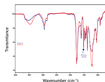
Figure 3. Comparison between two acetylated samples for a reaction time of 1 hour without catalyst (sample 01) and with catalyst (sample 08).
