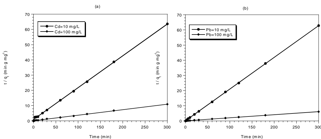
Figure 2 Pseudo second-order sorption kinetics of (a) Cd(II) and (b) Pb(II).
