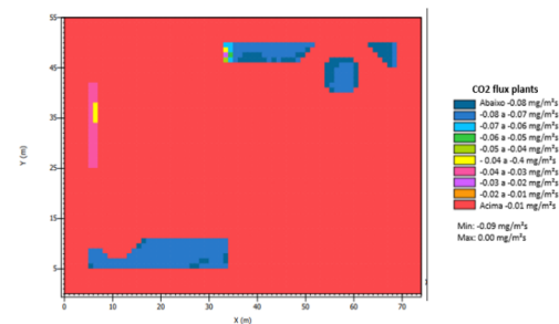
Fig. 5. CO 2 flux plants for scenario 0 in 2022.
