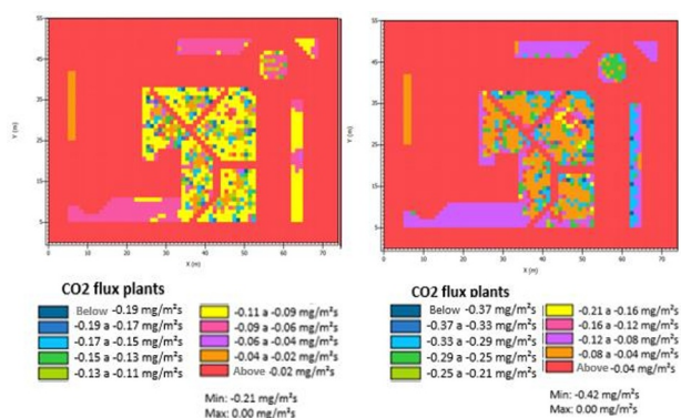
Fig. 7. CO 2 flux plants for scenario 2 in 2022 and 2052, respectively.
