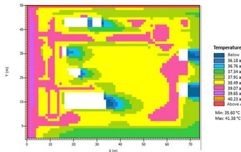
Fig. 8. Temperature for scenario 0 in 2022.
