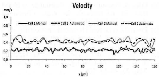
Figure 7. Velocity of two cells by using both methods.
