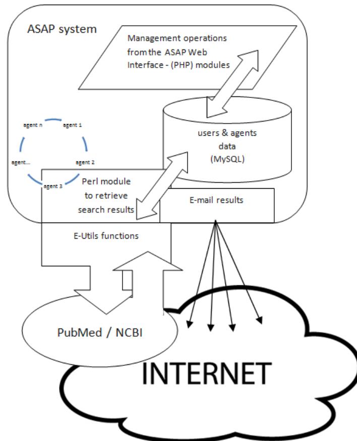
Fig.1 . The ASAP system's functional architecture.
