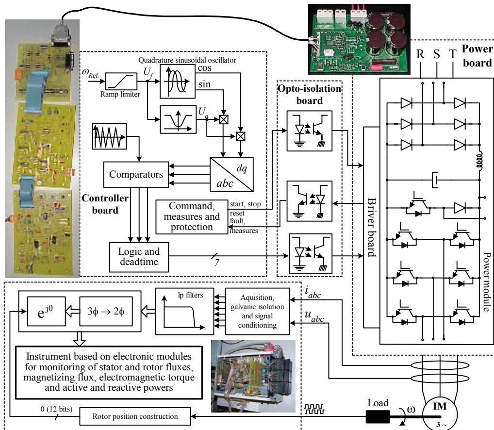
Fig. 1 – General diagram of the test bench prototype.
