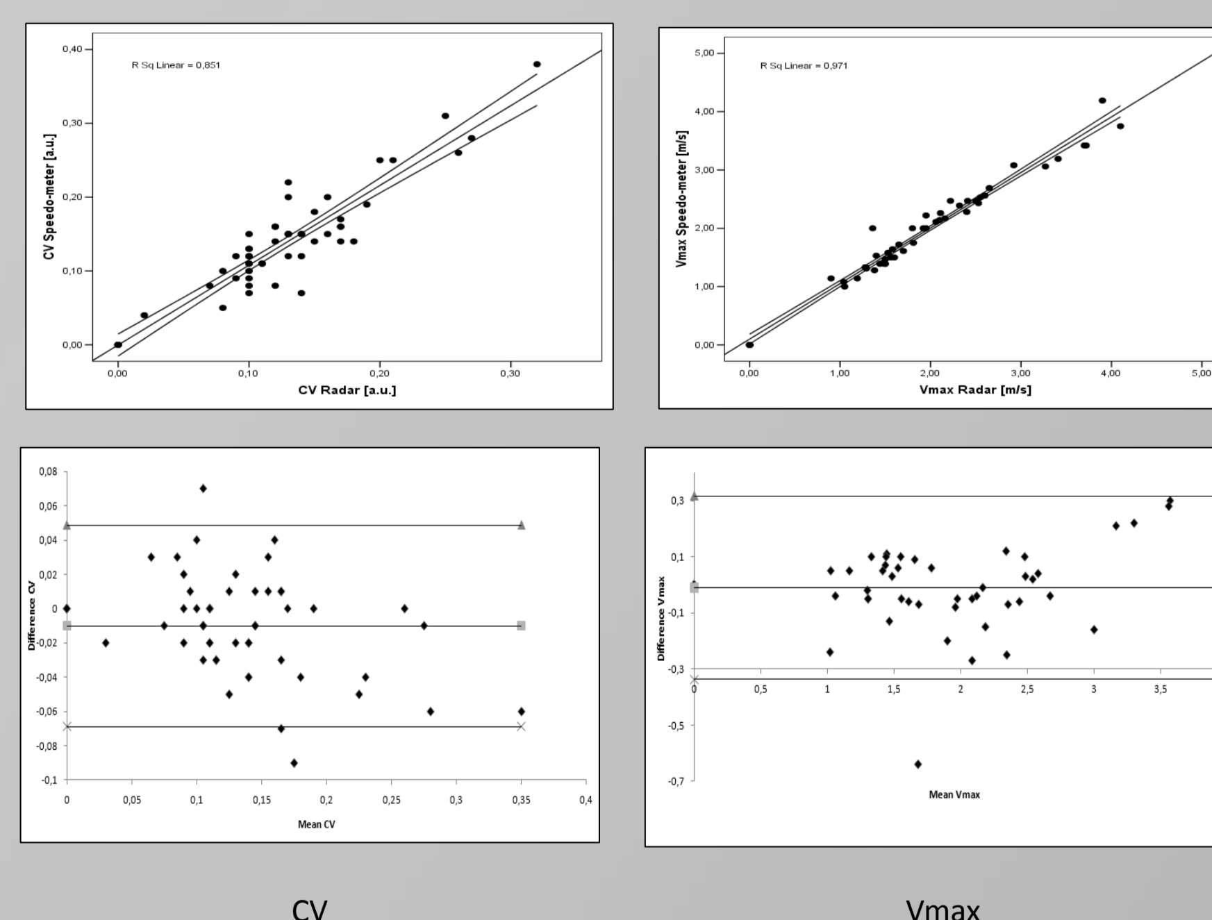
Figure 6. Linear regression models and Bland-Altman plots between speedo-meter system and radar gun coefficient of variation and maximal velocity within each gait cycle
