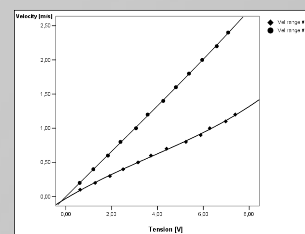
Figure 4. Relationship between DC tension and linear velocity
