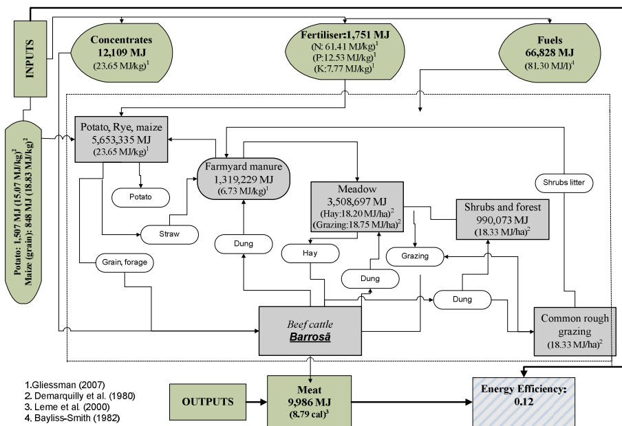
Figure 1. Flow diagram of the farm.
