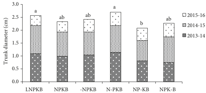
Figure 4. Average annual increase in trunk diameter of the young chestnut trees in the treatments corresponding to the application of lime (L) plus NPKB (LNPKB), NPKB without lime (NPKB), and the other nutrients without N (-NPKB), P (N-PKB), K (NP-KB), or B (NPK-B). Letters above the columns indicate the results of the Tukey HSD test ( \alpha = 0.05 ) for the total trunk diameter increase from 2013 to 2016.
