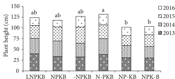
Figure 3. Average annual increase in height of the young chestnut trees in the treatments corresponding to the application of lime (L) plus NPKB (LNPKB), NPKB without lime (NPKB), and the other nutrients without N (-NPKB), P (N-PKB), K (NP-KB), or B (NPK-B). Letters above the columns indicate the results of the Tukey HSD test ( \alpha = 0.05 ) for the total height of plants.
