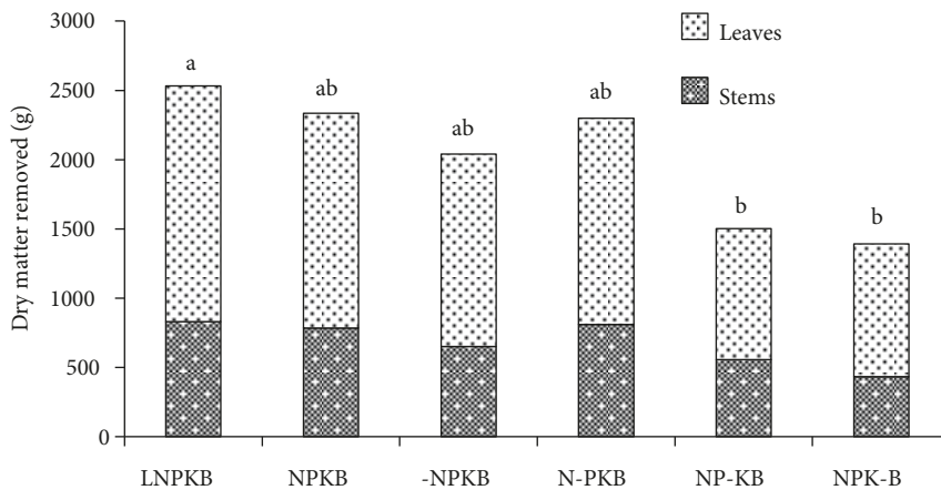
Figure 5. Average sum (2014-2016) of prunings separated into stems and leaves in the treatments corresponding to the application of lime (L) plus NPKB (LNPKB), NPKB without lime (NPKB), and the other nutrients without N (-NPKB), P (N-PKB), K (NP-KB), or B (NPK-B). Letters above the columns indicate the results of the Tukey HSD test ( \alpha = 0.05 ) for the total trunk diameter increase from 2013 to 2016.
