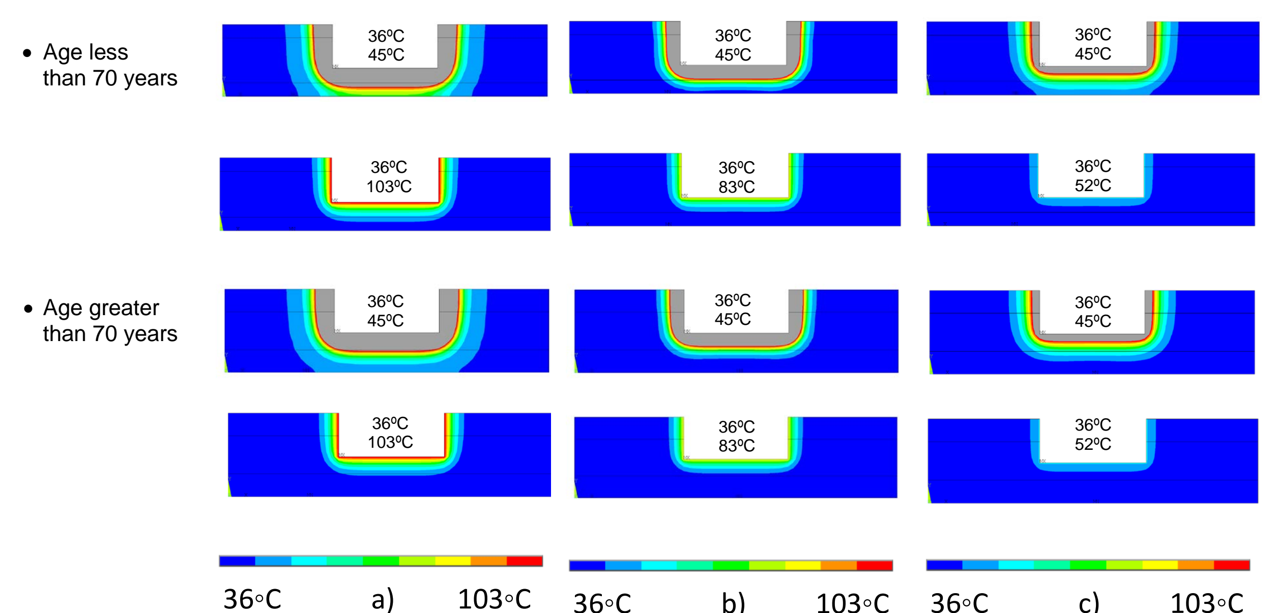
Figure 5 –Thermal analysis, function of: a) Curve A, b) Curve B, c) Curve C.
