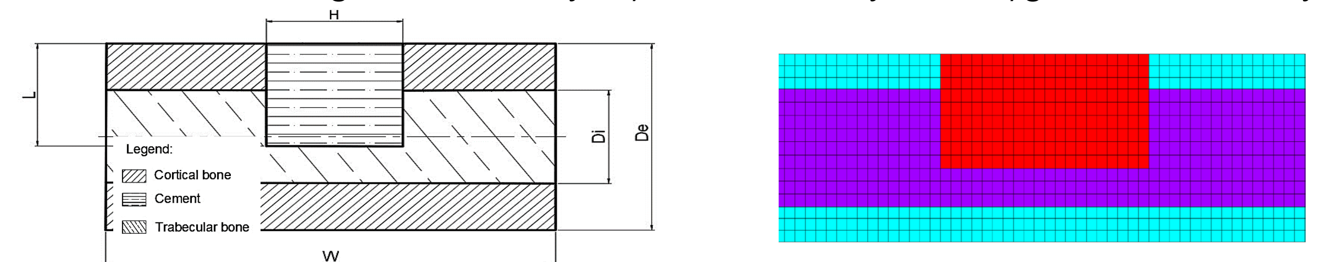
Figure 3 –Representative drawing and computational model.
