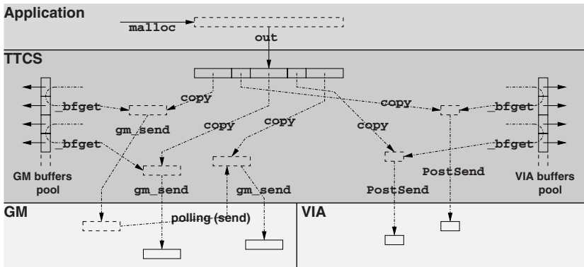
Fig. 3. Fragment dispatching.
