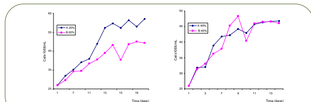
Fig 2. Growth of C. vulgaris in batch cultures with 20% and 40% of diluted OMWW (A and B - essays duplicates).
