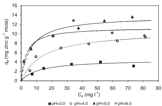
Fig. 4. Zinc sorption equilibrium isotherms at different pH values (moss concentration = 2 mg ml -1 ; T = 20^\circ\text{C} ; water hardness = 101.0 mg CaCO 3 l -1 ): experimental results and model fitting.
